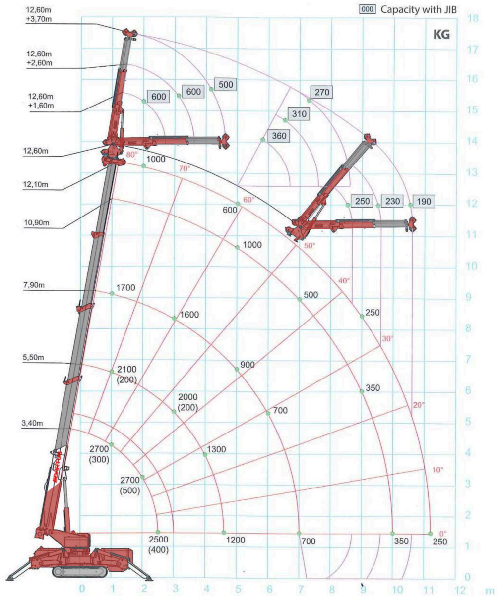
Load Chart
